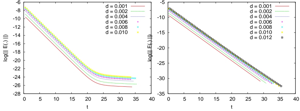
FIGURE 4.1. Large time behavior of the logarithm of the norm of the electric field, with two different numerical methods — the second one is supposed to be more accurate. The interaction is gravitational, the initial datum is a Gaussian multiplied by 1 + \varepsilon \cos(2\pi kx) .
