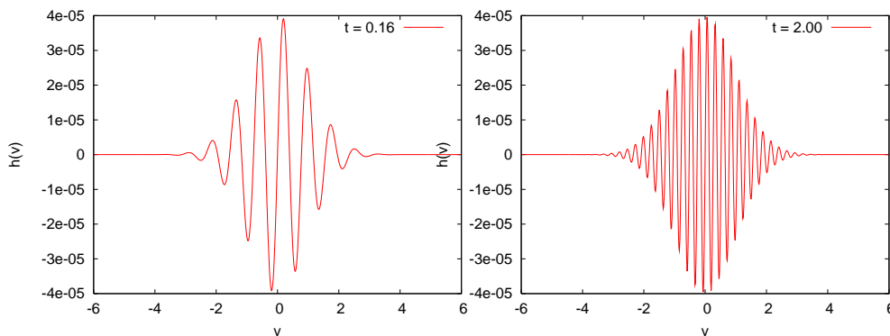
FIGURE 4.3. A plot of (f - f^0)(t, x, v) for some fixed x , as a function of v , at two different times t . The interaction is gravitational. Notice the fast oscillations of the distribution function, which are very difficult to capture by an experiment.
