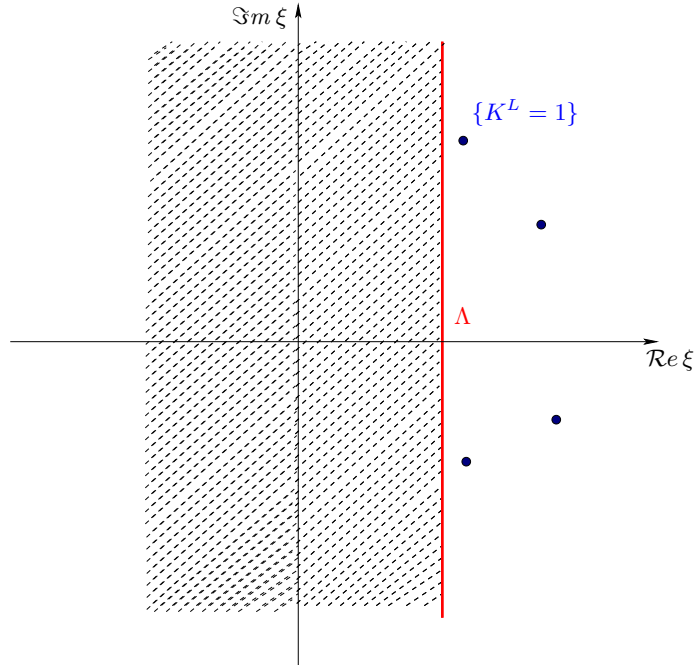
FIGURE 3.4. \Lambda > 0 is chosen so that the half plane \operatorname{Re} \xi \leq \Lambda contains no complex root of \{K^L = 1\} .
