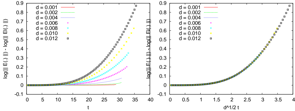
FIGURE 4.2. With the more accurate method from Figure 4.1, a plot of \log(\|E_{NL}\|/\|E_L\|) , the logarithmic ratio of the norm of the nonlinear electric field to the norm of the linearized electric field. On the left the time-scale is 1, on the right the time scale is 1/\sqrt{\varepsilon} . Here we see that we arrive in a time regime where the nonlinearity can definitely not be neglected.
